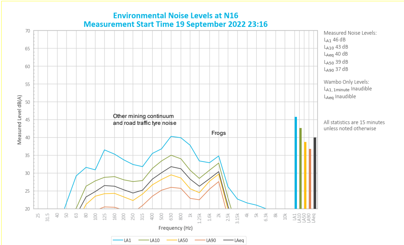
Figure 5.3 Environmental Noise Levels, N16 – Jerrys Plains Road
